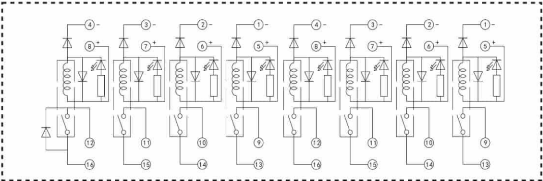
Wiring Diagram
