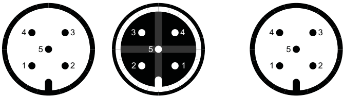
digital: plug connector/female connector - view from outside
