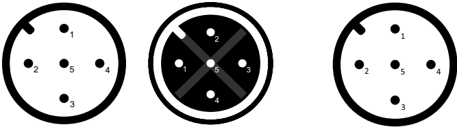
digital: plug connector/female connector - view from outside
