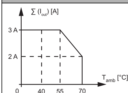
BWU2594, BWU2713, Derating total current of outputs
