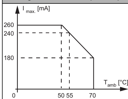
BWR1218 Derating total current of inputs/outputs
