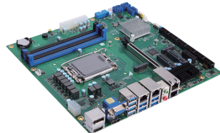
▲ DDR5 Side view
